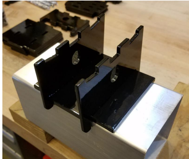
2. Insert Side Plates into outermost Slots of Base Plate. Long Tabs go toward Bumper.
