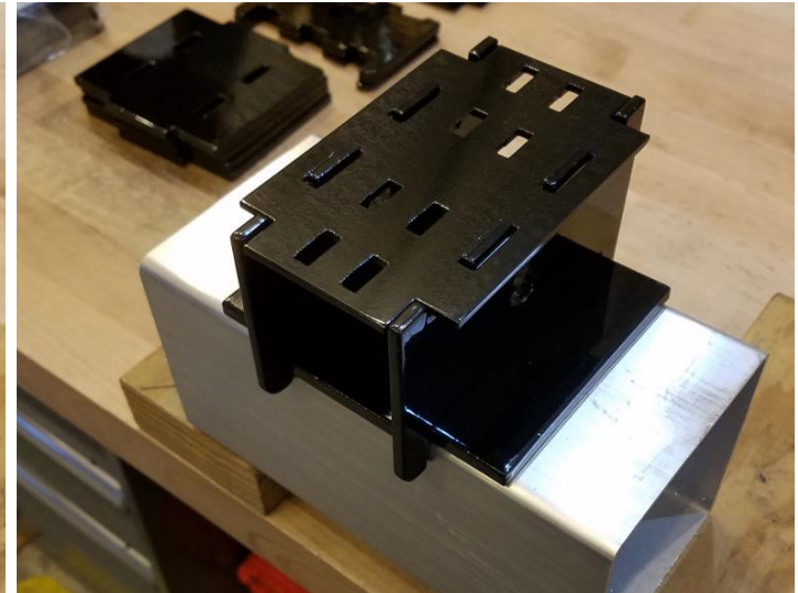
3. Set Pressure Plate atop Side Plates using outermost Slots in Pressure Plate.
